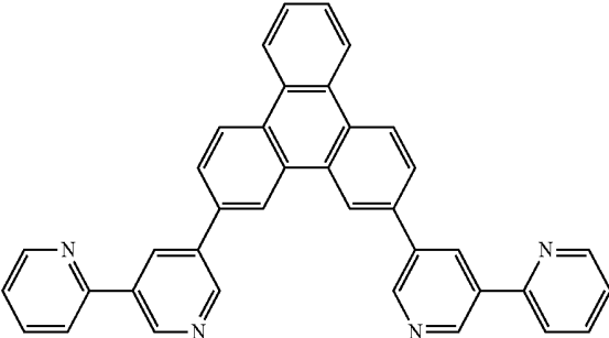
(Compound 16)
