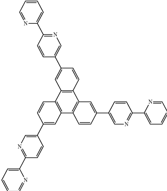
(Compound 17)
