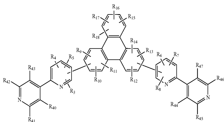
[Chemical Formula 6]
