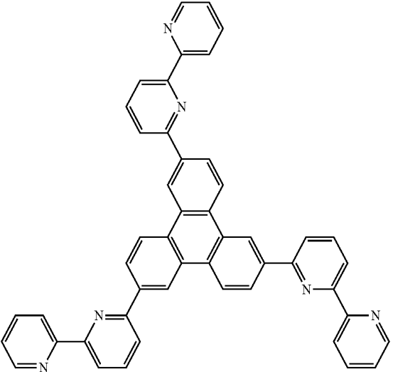
(Compound 18)
