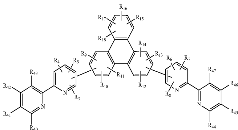
[Chemical Formula 5]
